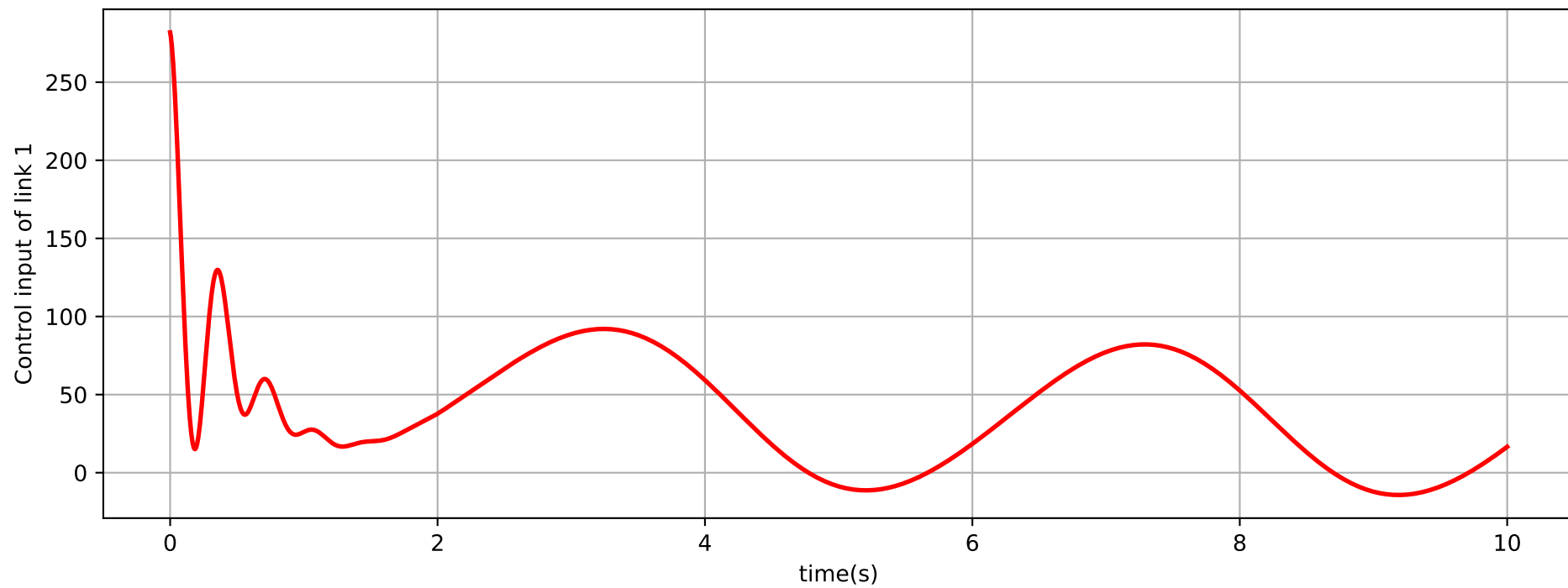
Control Inputs ( S=3 , S1=1 , m=5 )
